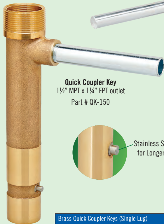
Quick Coupler Key 3/4" MPT x 1/2" FPT outlet Part # QK-075
